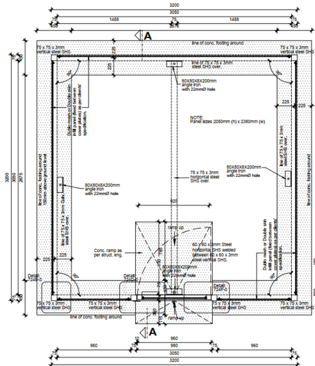
PLAN scale - 1:20
